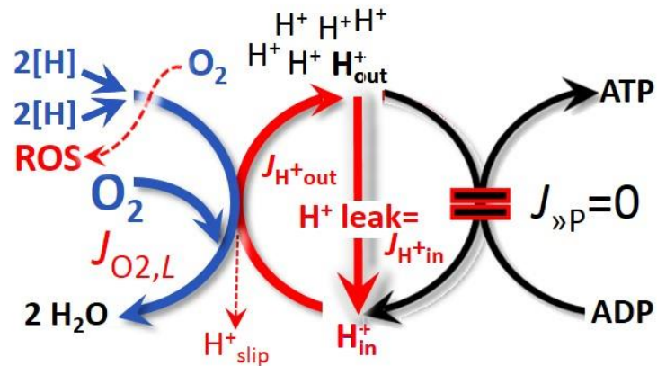
Fig. 5. LEAK state when phosphorylation is arrested, J_{\gg P}=0 , and oxygen flux, J_{O_2,L} , is controlled mainly by the proton leak, which equals J_{H^+in} , at maximum \Delta p_{mt} (compare Fig. 2).
